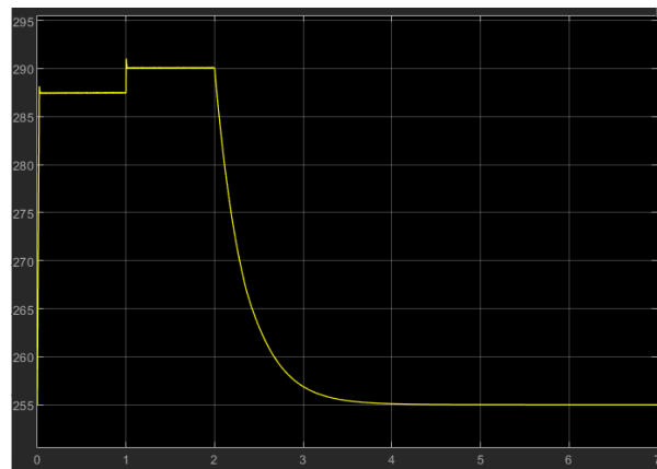
Figure (12) the temperature curve
