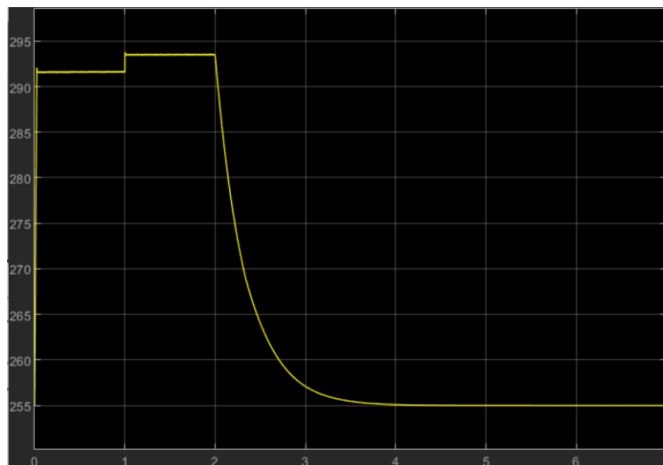
Figure (10) the temperature curve after tuning
