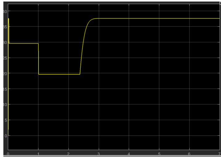
Figure (11) the output curvature with decreased load
